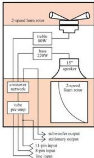
Diagram of model 3300
